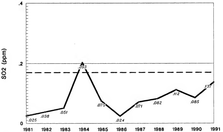
Figure 9.2 Maximum Hourly SO 2 Air Quality Data, Coronach Water Treatment Plant, 1981 to 1991, (Saskatchewan 1-hour standard).
